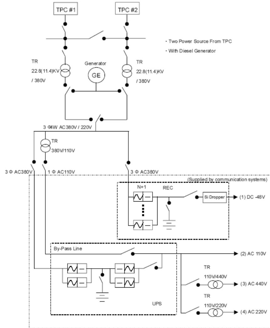
Fig.2.2.1.2 Configuration of Communication Power Supply at Station
